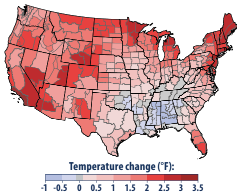
Rising temperatures in the last century. New Hampshire has warmed twice as much as the rest of the contiguous 48 states. Source: EPA, Climate Change Indicators in the United States .
